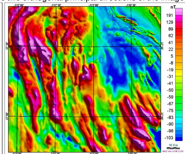
Figure 2. Total magnetic intensity of the study area
